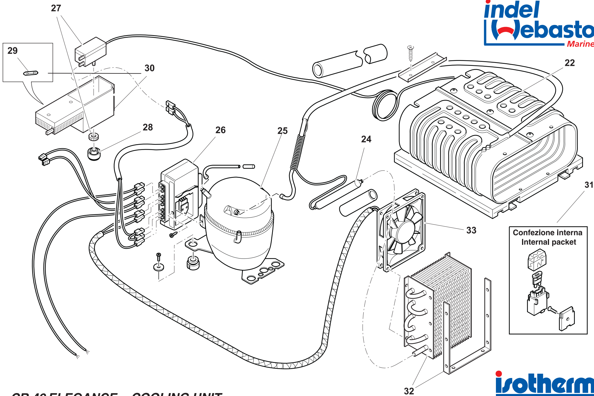
CR 49 ELEGANCE - COOLING UNIT
