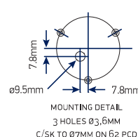
68000888 Stainless Steel Foot Switch
