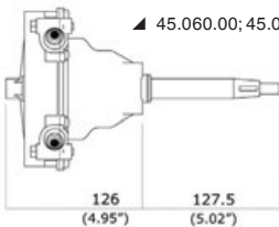
▲ 45.060.00; 45.061.00
